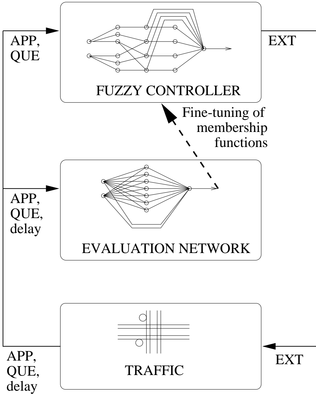
Figure 3: The neurofuzzy traffic signal control system.
