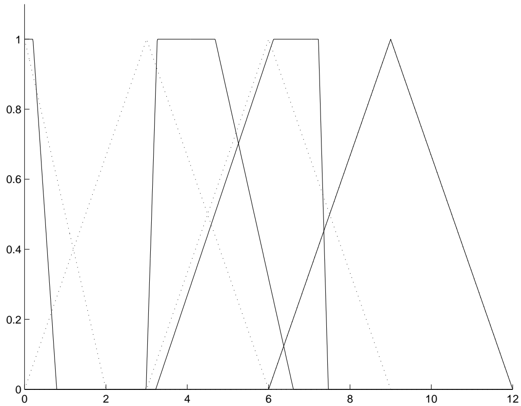
Figure 11: Membership functions zero , short , medium and long of EXT before (dotted line) and after (solid line) the learning at a traffic volume of 500 vehicles per hour. The location of the first traffic detector is 50 m from the stop line. Horizontal axis: green signal extension in seconds. Vertical axis: value of membership function.
