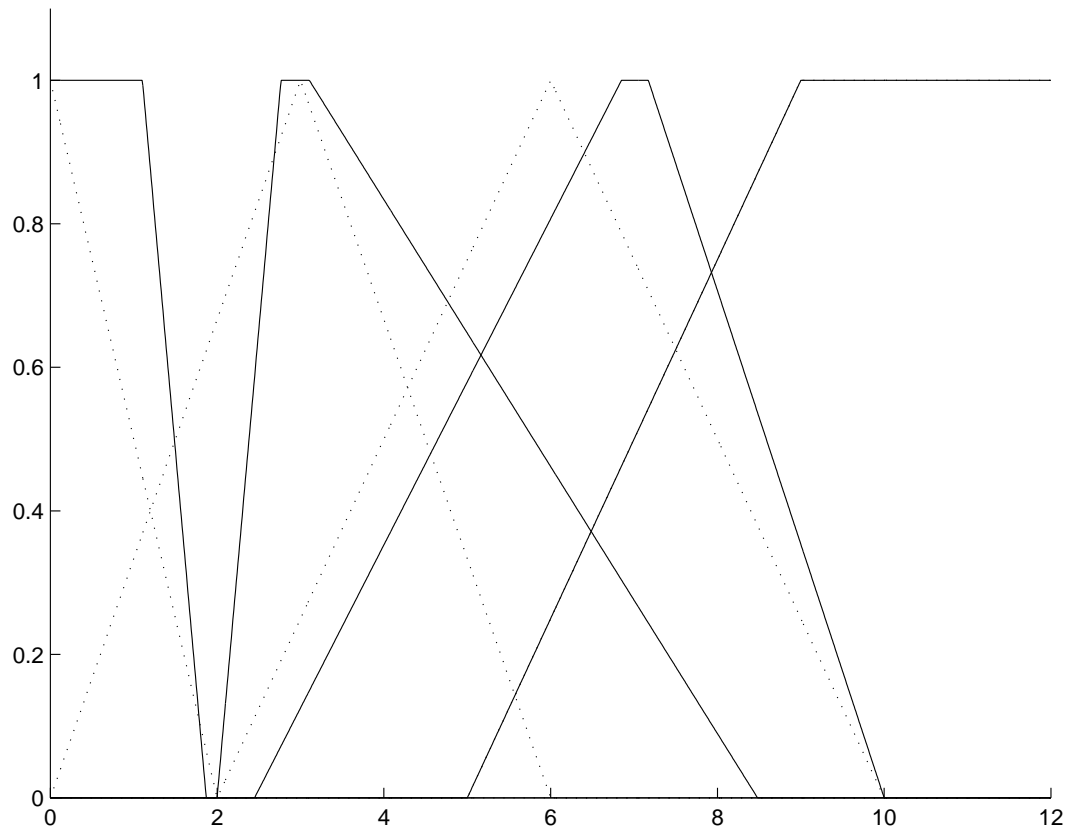
Figure 9: Membership functions zero , a few , medium and many of APP before (dotted line) and after (solid line) the learning at a traffic volume of 500 vehicles per hour. The location of the first traffic detector is 50 m from the stop line. Horizontal axis: number of approaching vehicles. Vertical axis: value of membership function.
