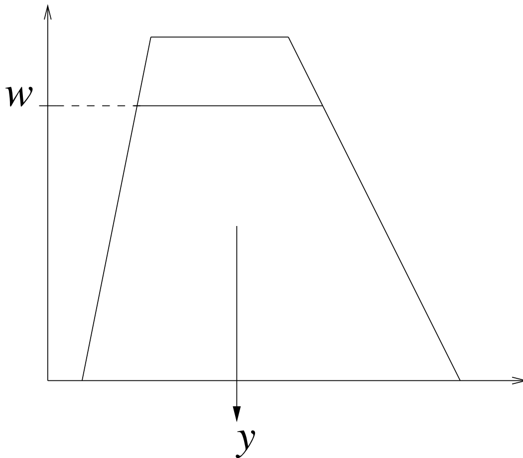
Figure 6: The membership function in the then-part of the rule is cut at the level indicated by the rule firing strength w . The output y of the rule is the center of area of the remaining set.
