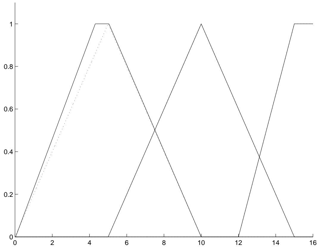
Figure 10: Membership functions a few , medium and too long of QUE before (dotted line) and after (solid line) the learning at a traffic volume of 500 vehicles per hour. The location of the first traffic detector is 50 m from the stop line. Horizontal axis: number of queuing vehicles. Vertical axis: value of membership function.
