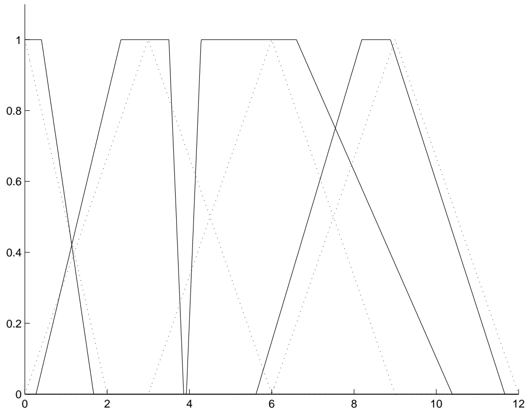
Figure 13: Membership functions zero , short , medium and long of EXT before (dotted line) and after (solid line) the learning at a traffic volume of 500 vehicles per hour. The location of the first traffic detector is 100 m from the stop line. Horizontal axis: green signal extension in seconds. Vertical axis: value of membership function.
