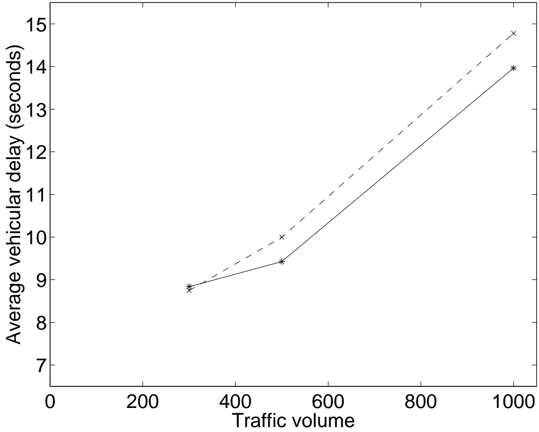
Figure 7: Average vehicular delays (in seconds) before (dashed line) and after (solid line) the learning at traffic volumes of 300, 500 and 1000 vehicles per hour. The location of the first traffic detector is 50 m from the stop line.
