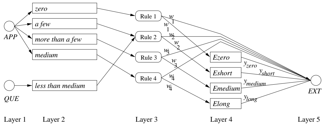
Figure 5: Fuzzy traffic signal controller presented as a neural network. The first rule set of the rule base.
