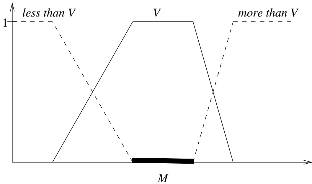
Figure 2: Membership functions for linguistic values V , less than V and more than V . The thick line shows M (Formula (1)).
