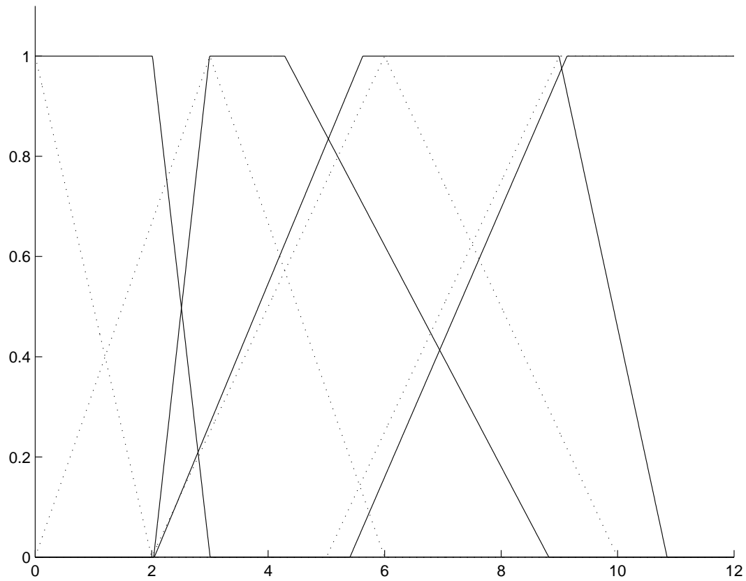
Figure 12: Membership functions zero , a few , medium and many of APP before (dotted line) and after (solid line) the learning at a traffic volume of 1000 vehicles per hour. The location of the first traffic detector is 50 m from the stop line. Horizontal axis: number of approaching vehicles. Vertical axis: value of membership function.
