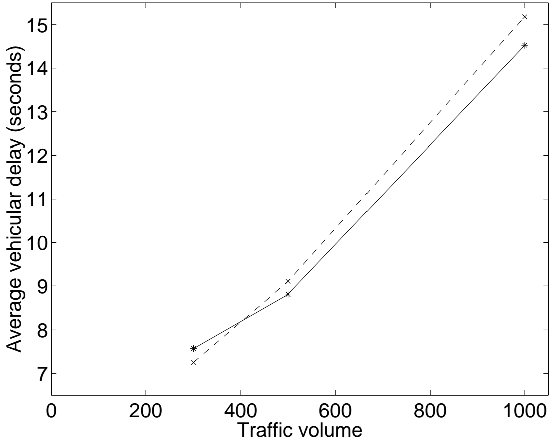
Figure 8: Average vehicular delays (in seconds) before (dashed line) and after (solid line) the learning at traffic volumes of 300, 500 and 1000 vehicles per hour. The location of the first traffic detector is 100 m from the stop line.
