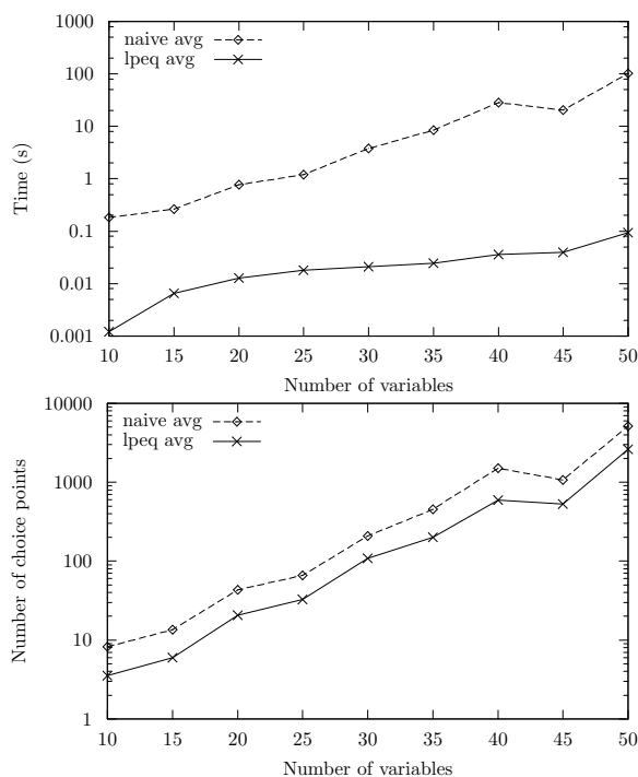
Fig. 4. Average running times and numbers of choice points for random 3-sat instances with the ratio c/v = 4 .
