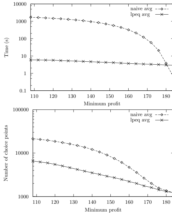
Fig. 7. Average running times and average number of choice points for knapsack.
